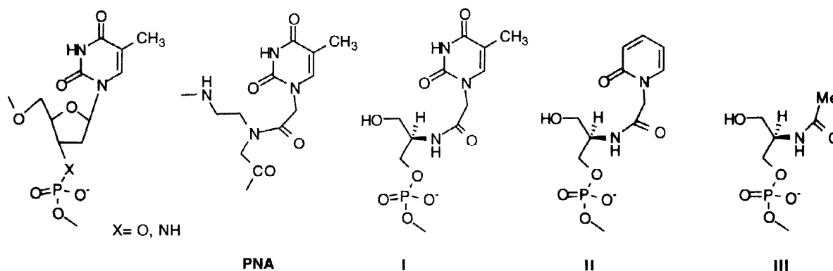
Scheme 1: Nucleotide analogues
